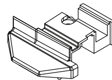
LM0388 2 Part 70mm Meeting Stile End Cap Chamfered Detail
