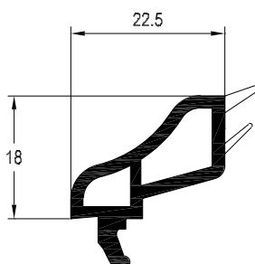
Co-extruded Glazing Bead 22.5mm White Art. No. 551510 Laminated Art. No. 581580
