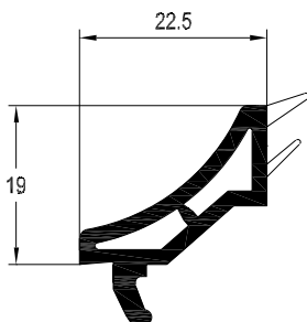
Co-extruded Glazing Bead 22.5mm White Art. No. 561450 Laminated Art. No. 576550*
